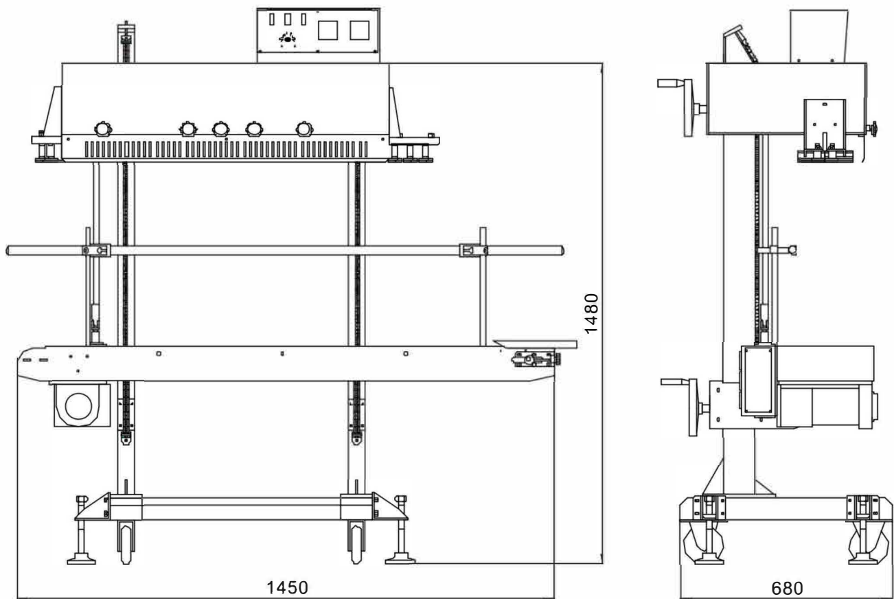
4-BS-PV100700+ Continuous band sealer with two sets of heating blocks Diagram 2
