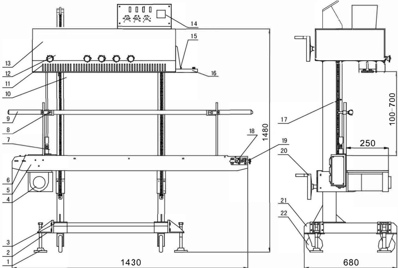
4-BS-PV100700 Solid - ink coding continuous band sealer
